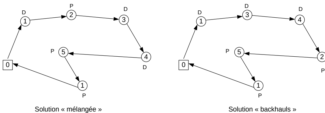
Figure 11 : Type de solution
