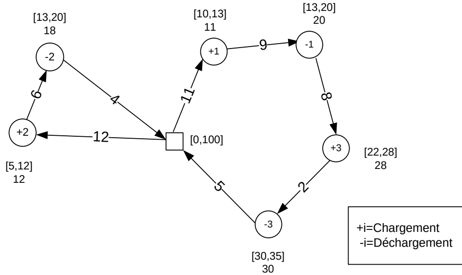
Figure 15 : VRPPDTW
