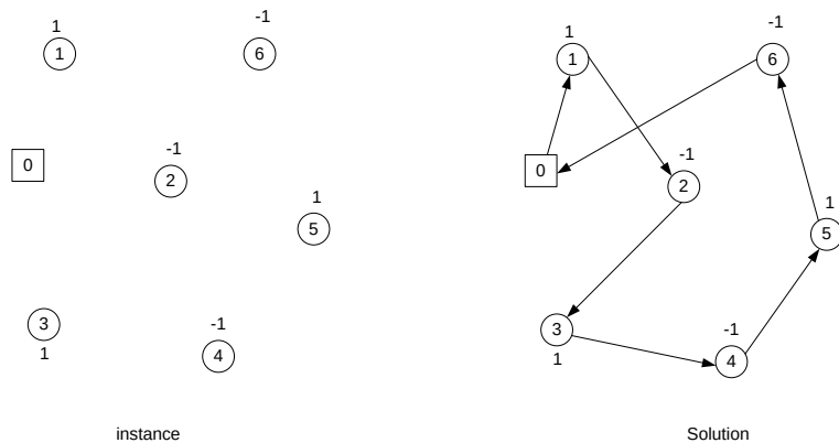
Figure 7 : Q-DTSP
