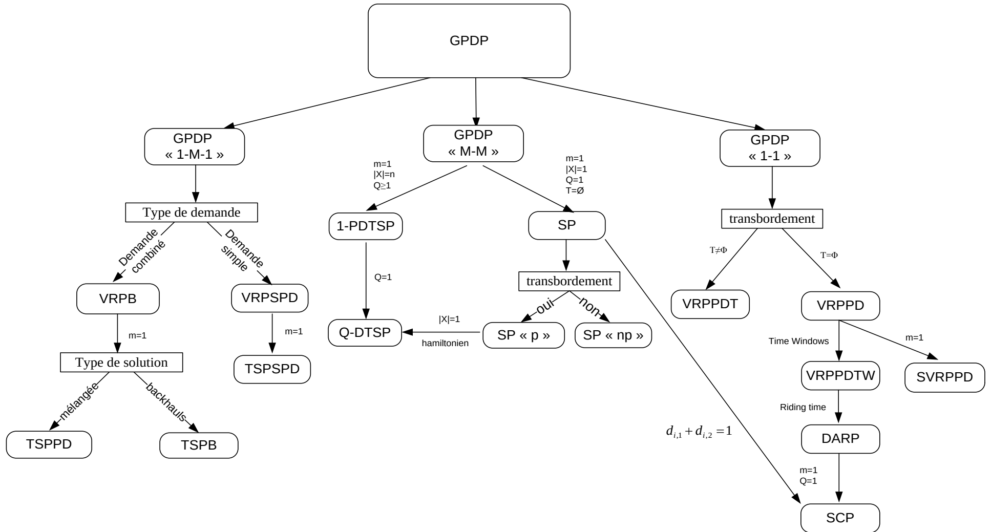
Figure 17 : Classification du GPDP
